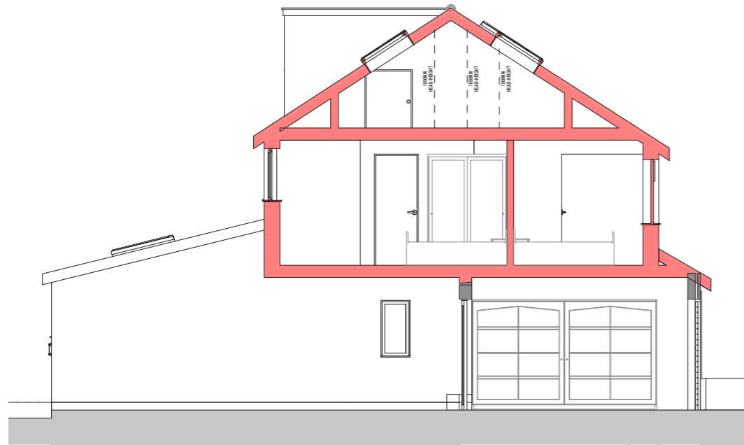
C Building Section 1:100
